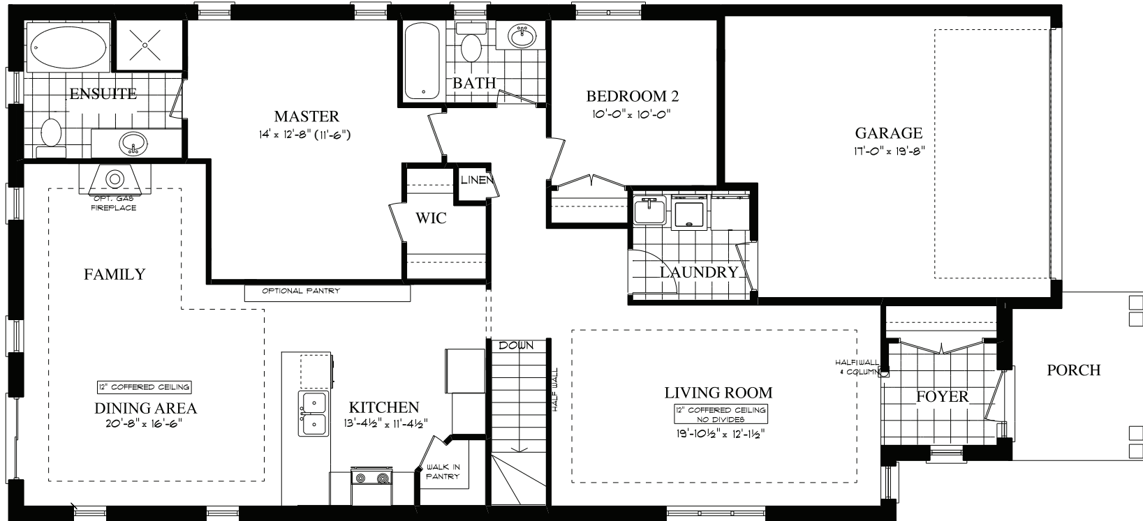
Main Floor Plan Floor Area - approx. 1585 sq. ft.
